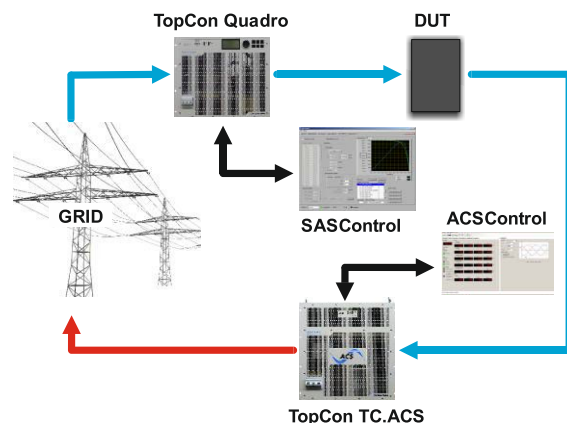
Fig.1 Example of a Solar Inverter test bench with grid simulator
