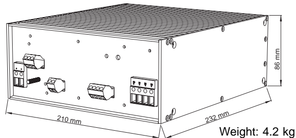
Figure 1. Dimensions
