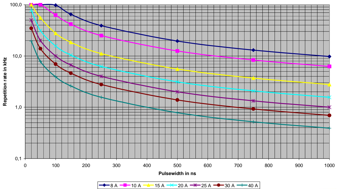
LDP-V 40-70: Max. Reprate vs. Pulsewidth
