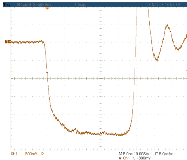
Typical Pulse Rise and Fall Times (scale: 10 A/Div)
